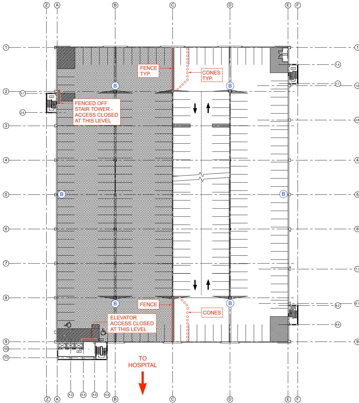
AS FOURTH LEVEL PLAN Scale: 1/16" = 1'-0"
