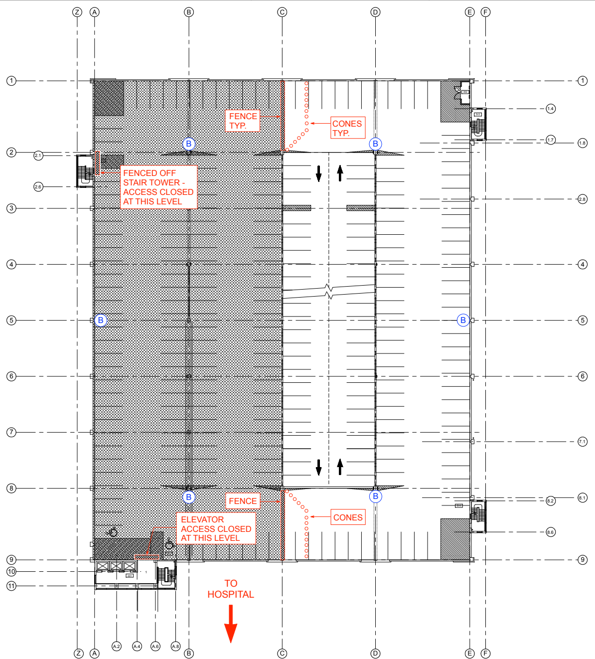
A3 THIRD LEVEL PLAN Scale: 1/16" = 1'-0"
